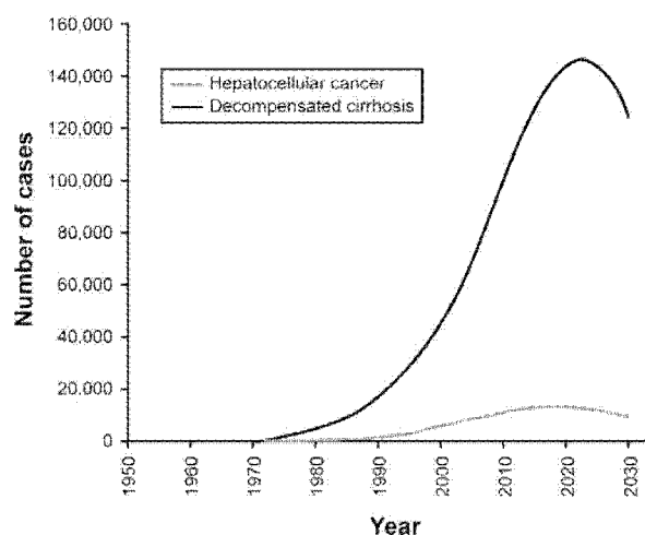
Figure 4. Projected number of cases by year of decompensated cirrhosis ( black ) and hepatocellular carcinoma ( gray ). The model assumes a first year mortality of 80% to 85%, so in contrast to the decompensated cirrhosis projection, the number of cases of hepatocellular carcinoma the prevalence demonstrated here closely resembles annual incidence of liver cancer.
